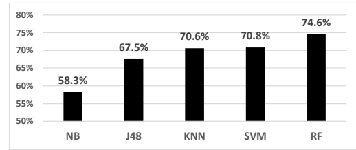
Figure 2. Comparison of the 5 ML algorithms: Naïve Bayes (NB), C4.5 Decision tree (J48), K-nearest neighbours (KNN), Support vector machines (SVM) and Randomf Forest (RF)
